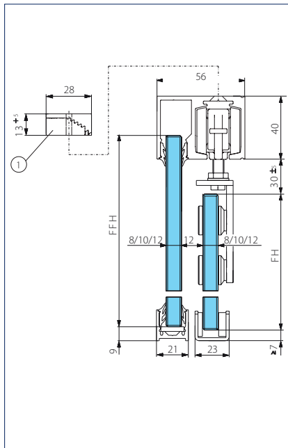
Fastpanelmontering glass
