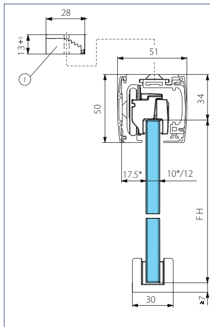
Takmontering glass
