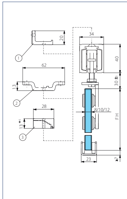
Vegg-/takmontering glass
