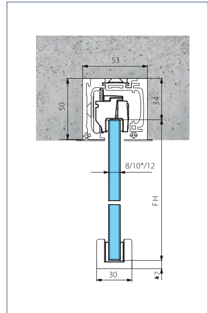
Takmontering glass
