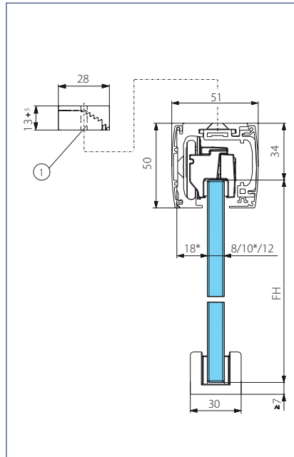
Takmontering glass
