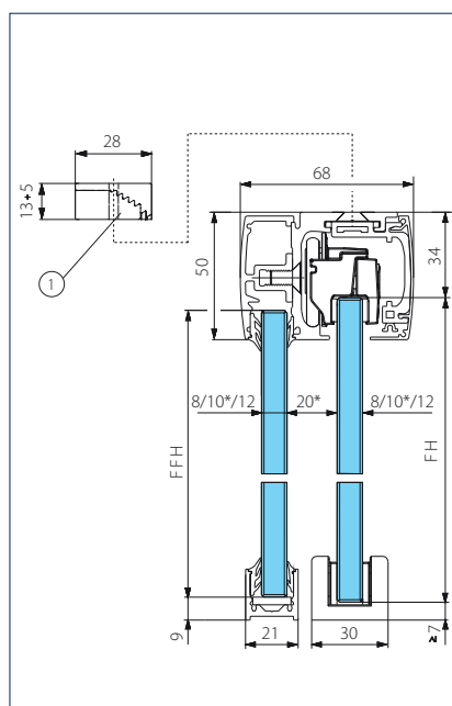
Fastpanelmontering glass
