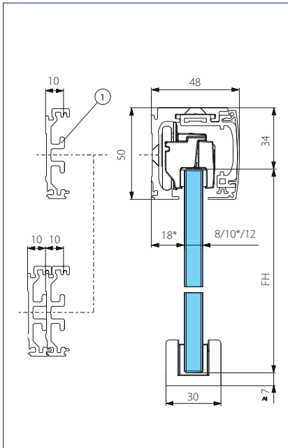
Veggmontering glass
