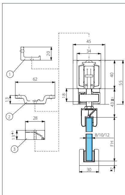
Vegg-/takmontering glass
