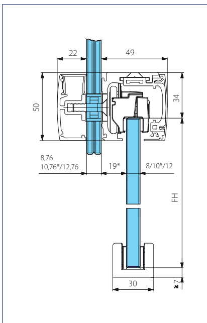
Overlysmontering glass
