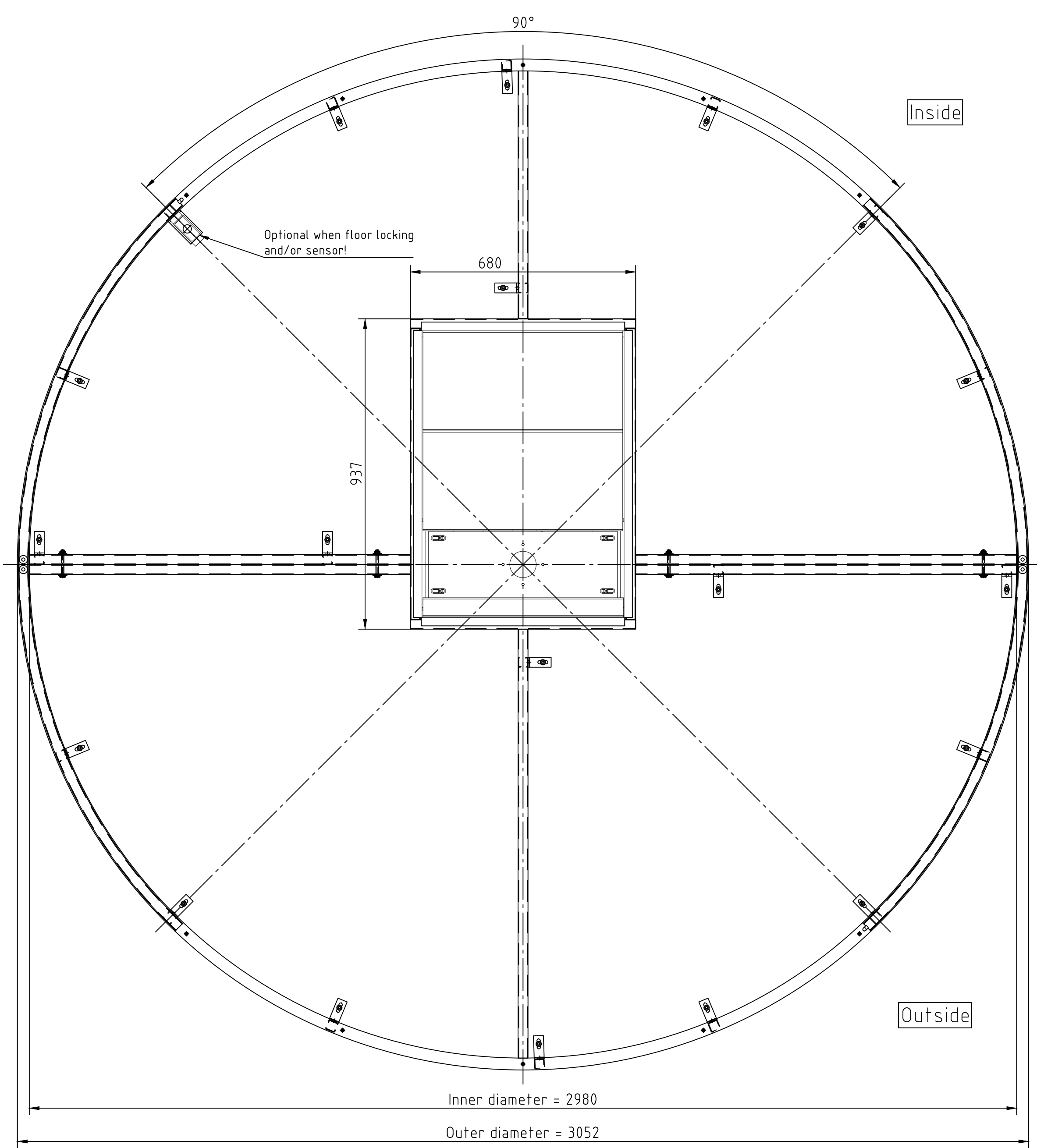
Floor ring GG-3lvs-UFA plan view
