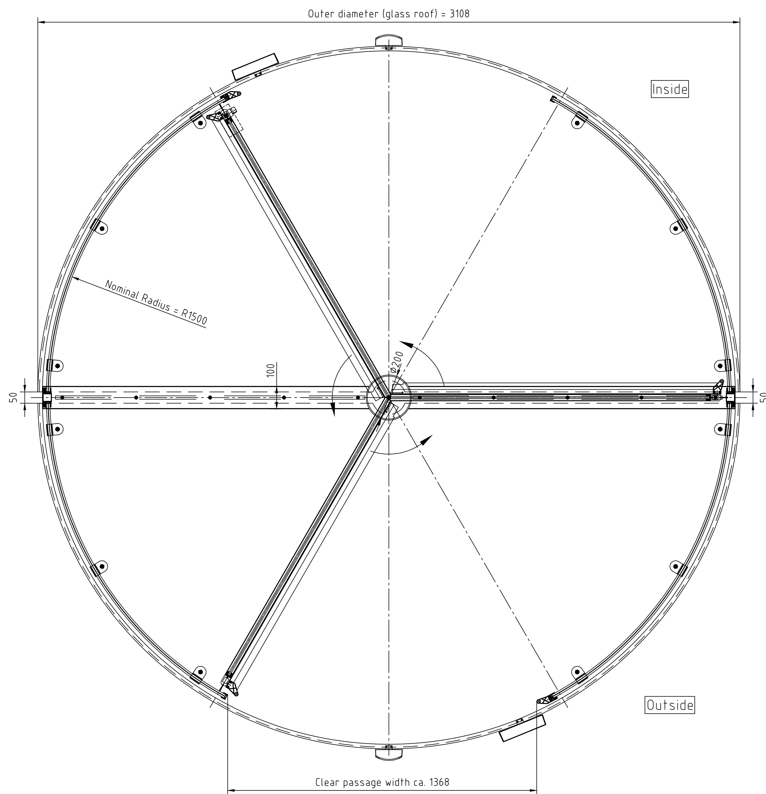
Revo.PRIME A3-GG-UFA plan view
