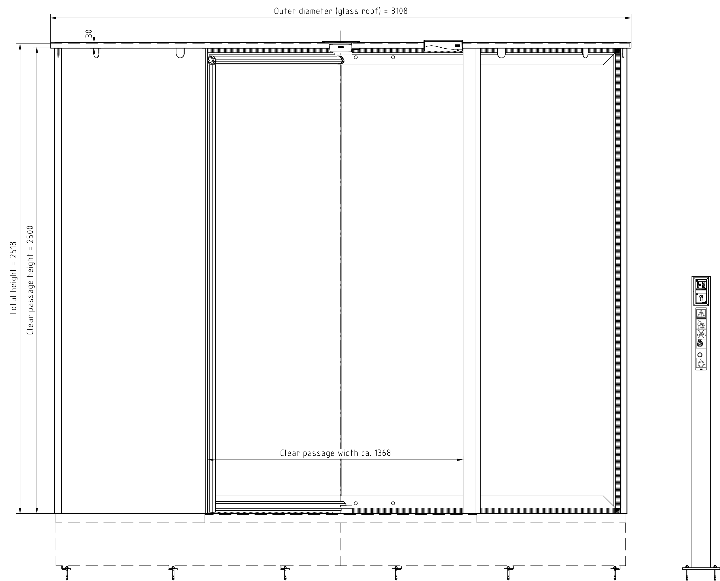
Revo.PRIME A3-GG-UFA front view
