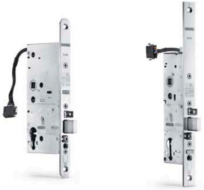
Mechanical contact lock with feedback contacts for single leaf doors
