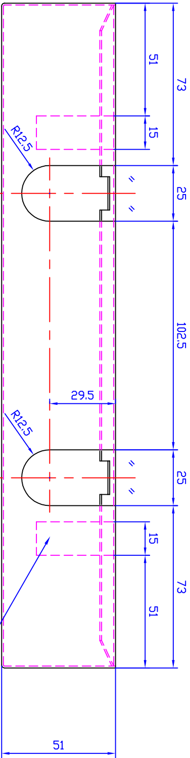
PLAN VIEW
