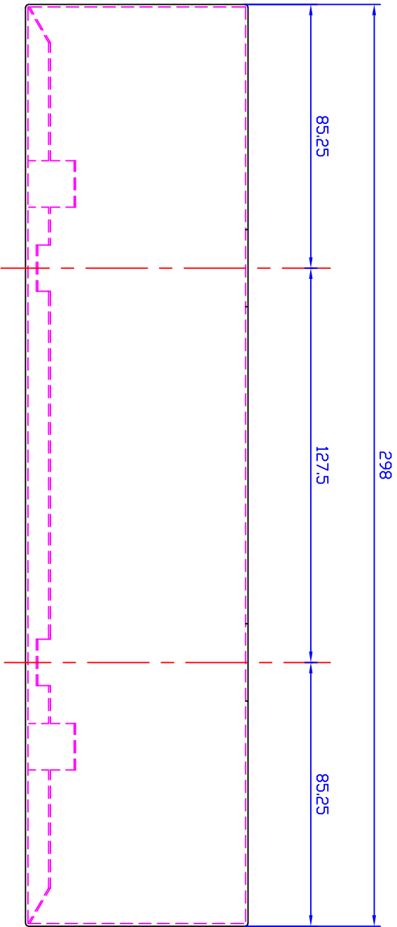
ELEVATION "B"
